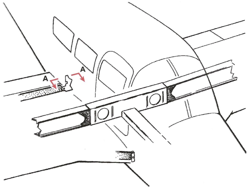
WING INSTALLATION ISOMETRIC VIEW
